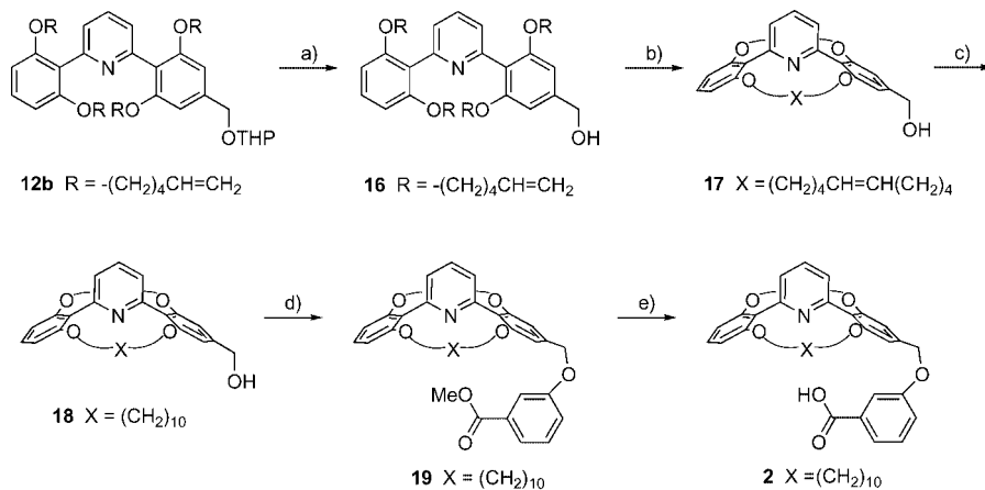
Scheme 4. a) p -TsOH, MeOH, reflux, 90 min; b) CH 2 Cl 2 , Grubbs' cat. (1st generation), room temp., 21 h; c) Pd/C, H 2 , MeOH, room temp., 18 h; d) THF, PPh 3 , diisopropyl azodicarboxylate (DIAD), methyl 3-hydroxybenzoate, 0 °C, room temp., 18 h; e) THF, MeOH, LiOH, H 2 O, 40 °C, 4 h, room temp., 18 h.
