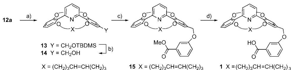
Scheme 3. a) CH 2 Cl 2 , Grubbs' cat. (1st generation), room temp., 48 h; b) THF, NBu 4 F·3H 2 O, room temp., 45 min; c) THF, PPh 3 , diisopropyl azodicarboxylate (DIAD), methyl 3-hydroxybenzoate, 0 °C → room temp., 18 h; d) THF, MeOH, LiOH, H 2 O, 40 °C, 4 h, room temp., 18 h.
